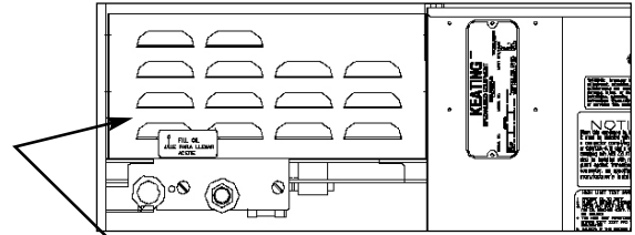
Remove the cover by loosening the screws to gain access to the burner viewing windows (14" Model Shown).
