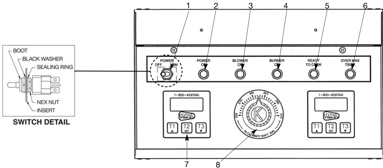
Back Panel (Front View)
