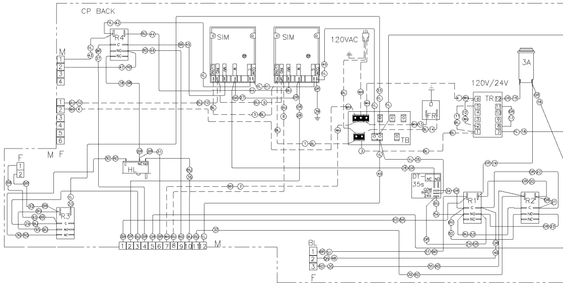
CONTROL PANEL BACK
