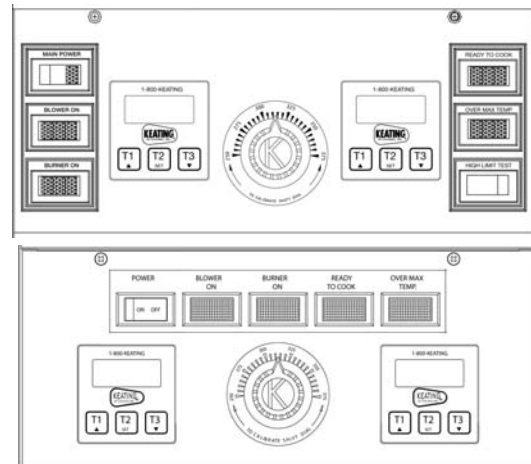
Control Panel with timers Model 2000
