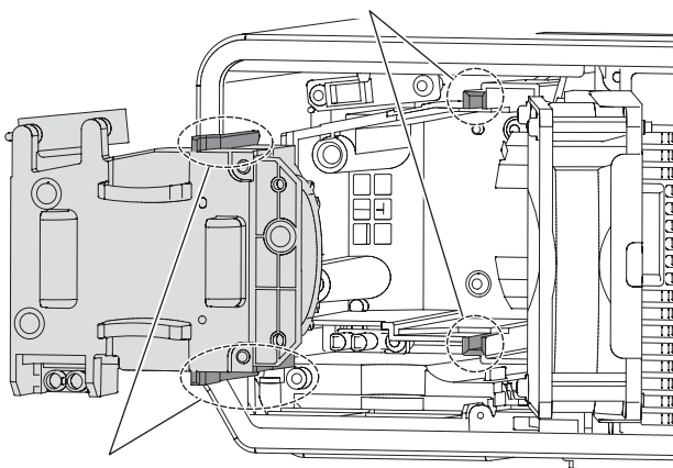
Lamp unit installation guide
