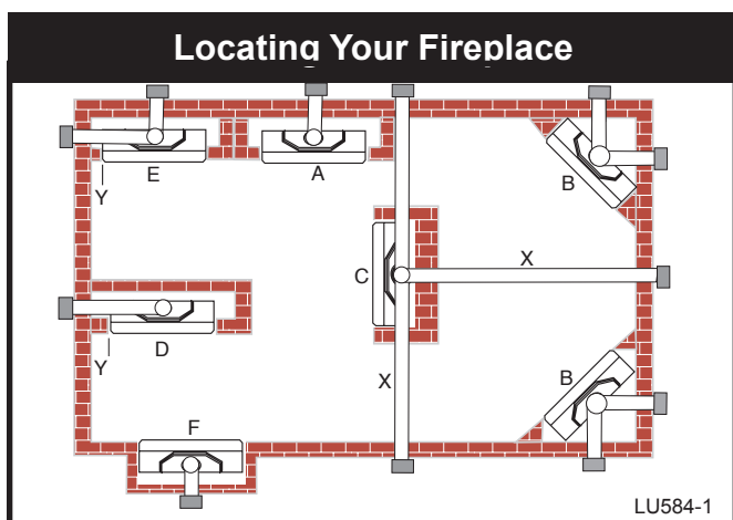
Fig. 2 Locate gas fireplace. A) Flat on wall B) Cross Corner C) As an Island D) As a room divider E) Flat on wall corner F) Exterior wall
