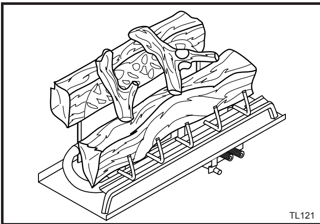
Fig. 34 DV1000 and DV1200 logs in final position.
