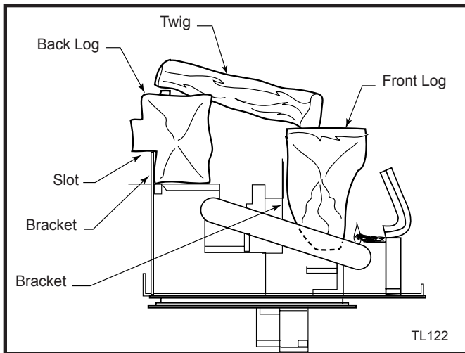
Fig. 35 Side view of logset. (NOTE: The side logs for the DV1400 are not shown.)
