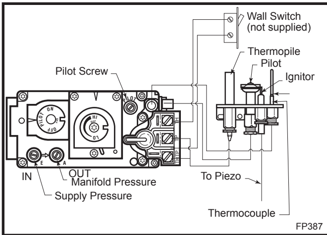
Fig. 37 Pilot and valve wiring.
