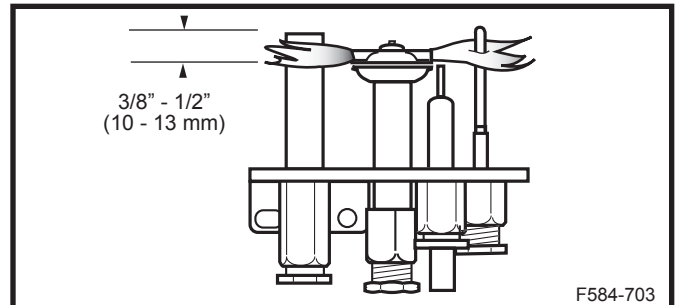
Fig. 39 Correct flame appearance.
