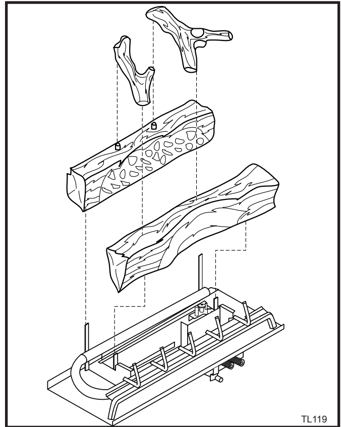
Fig. 32 Correct log placement for DV1000 and DV1200.
