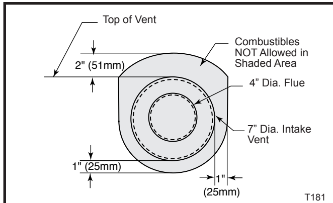
Fig. 11 Vent clearances.
