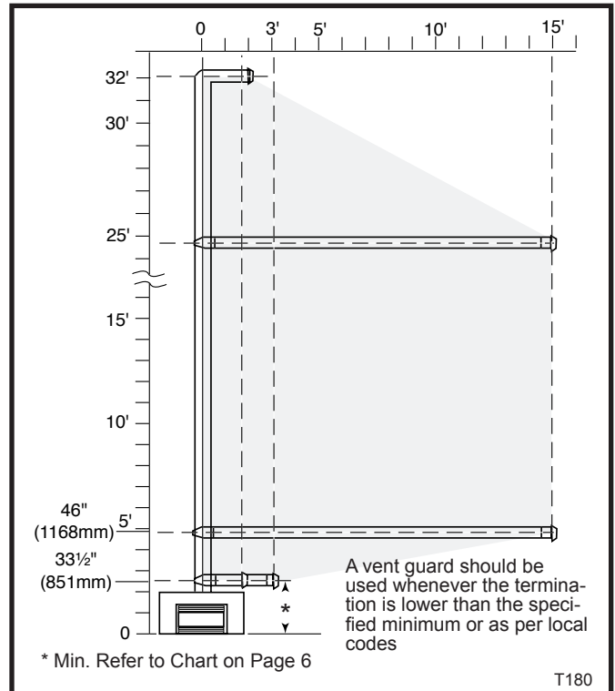
Fig. 12 Venting graph.
