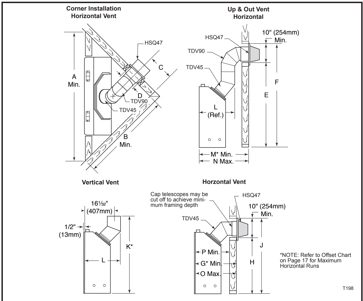
Fig. 29 Typical TDV Series vent applications.
