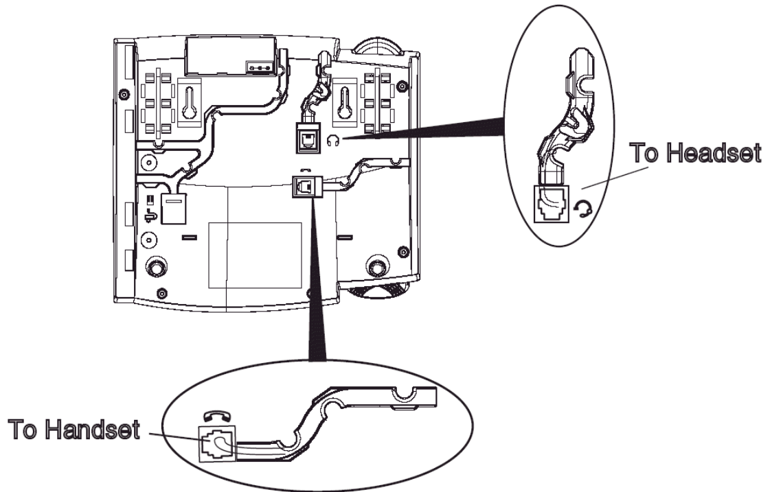
Figure 2 Headset and Handset Connection
