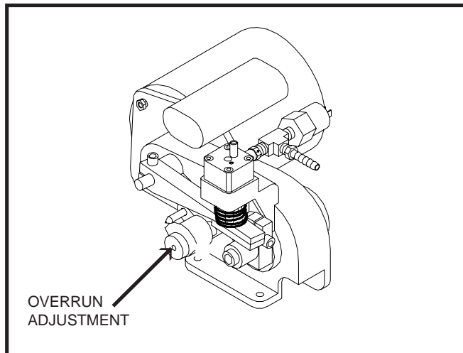
Figure 7 Overrun Adjustment
