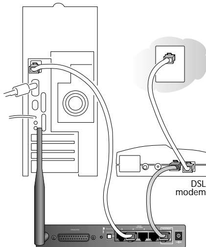
Model FM114P ProSafe Wireless Firewall with Print Server
