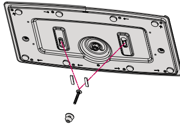
2-Screws, 2-Washers, 2-Nuts, 4-Rubber (provided as parts of the product)
