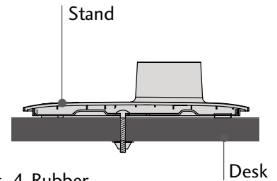
2-Screws, 2-Washers, 2-Nuts, 4-Rubber (provided as parts of the product)
