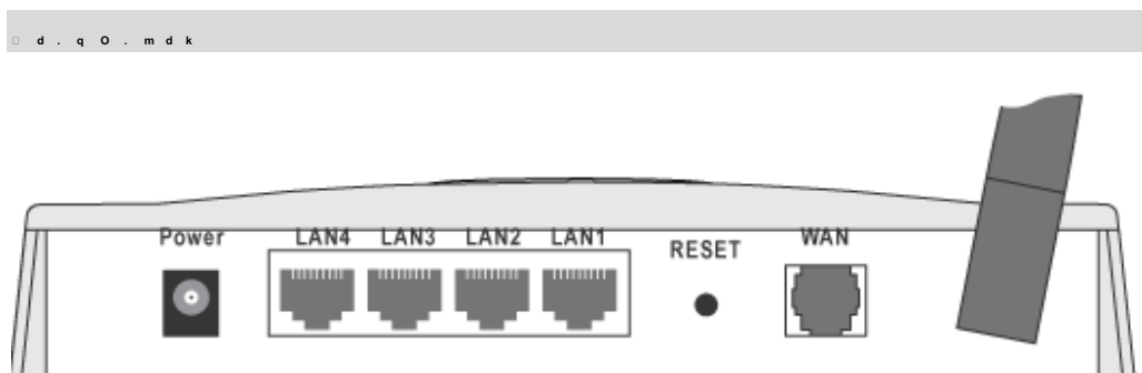
Figure 3: Rear Panel
