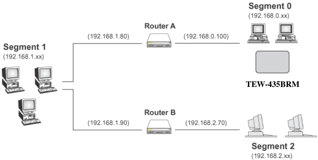
Figure 47: Routing Example
