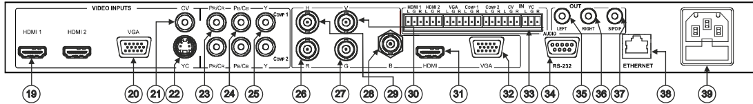
Figure 2: VP-441 Presentation Switcher/Scaler Rear Panel
