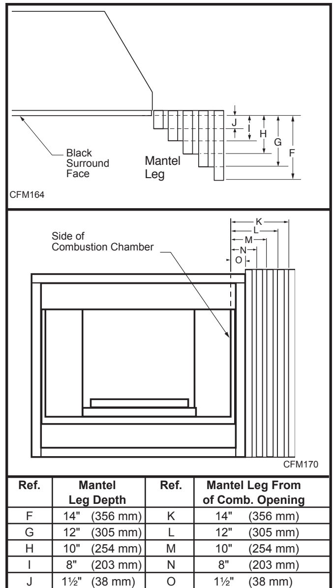
Fig. 3b Combustible mantel leg minimum installation.
