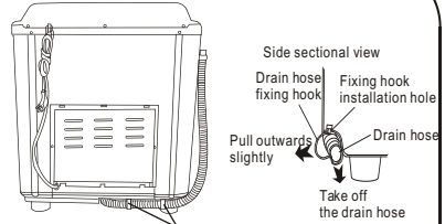
Figure 1 Drain hose fixing hook
