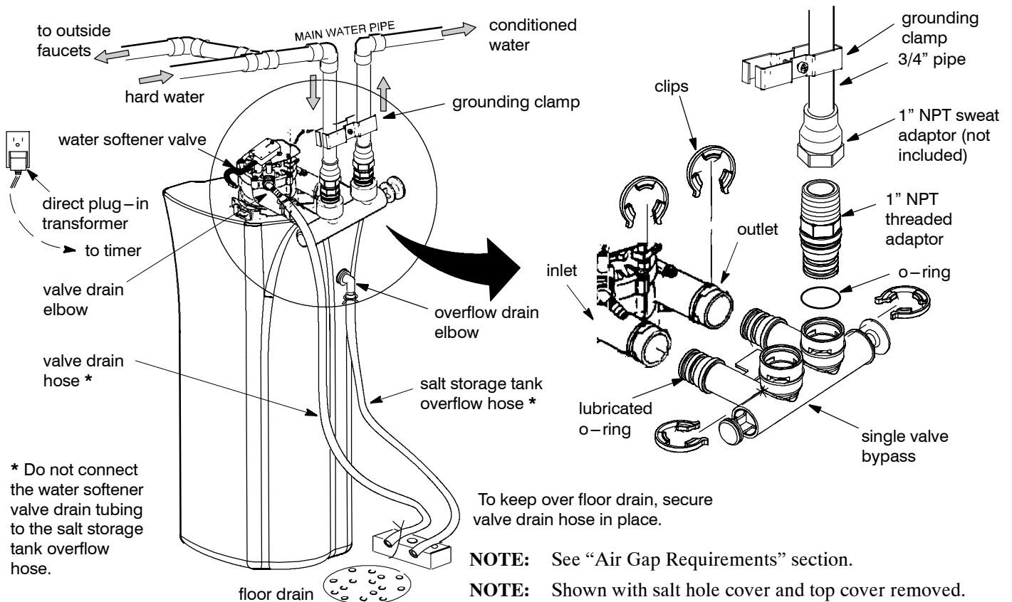
Figure 5 (typical installation)
