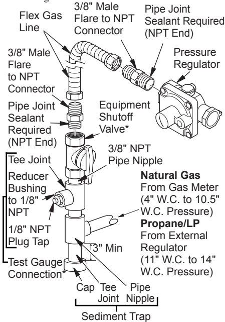
Figure 11 - Gas Connection
