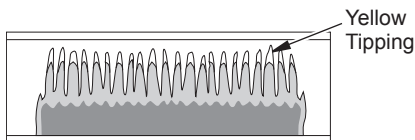
Figure 21 - Incorrect Burner Flame Pattern
