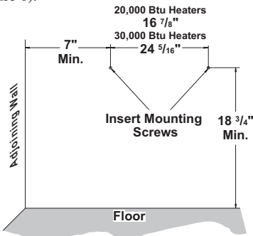
Figure 6 - Wall Mounting Clearances
