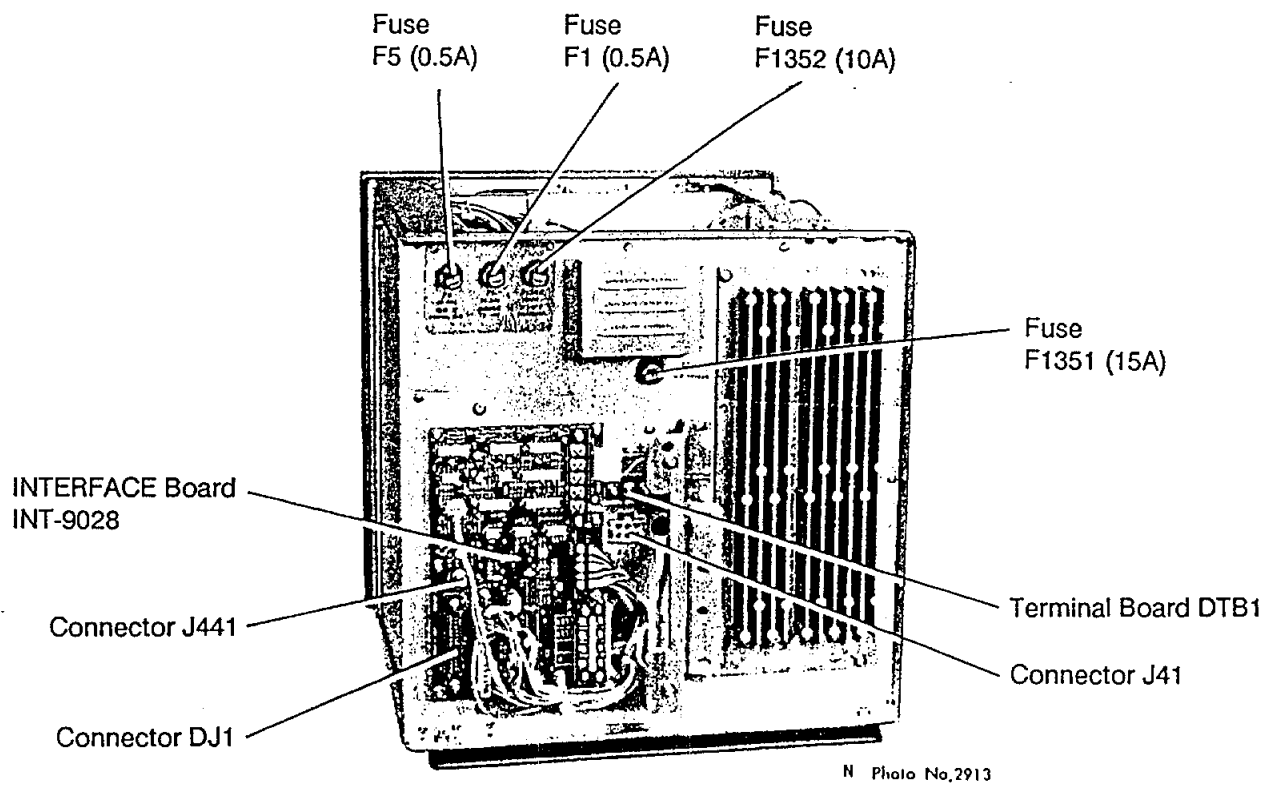
Figure 5-6 Display Unit, rear view
