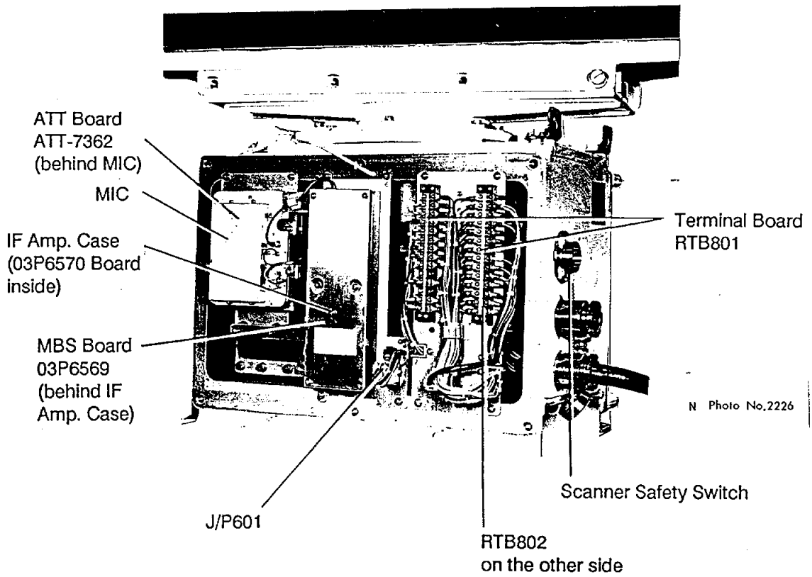
Figure 5-7 Scanner Unit, left side view
