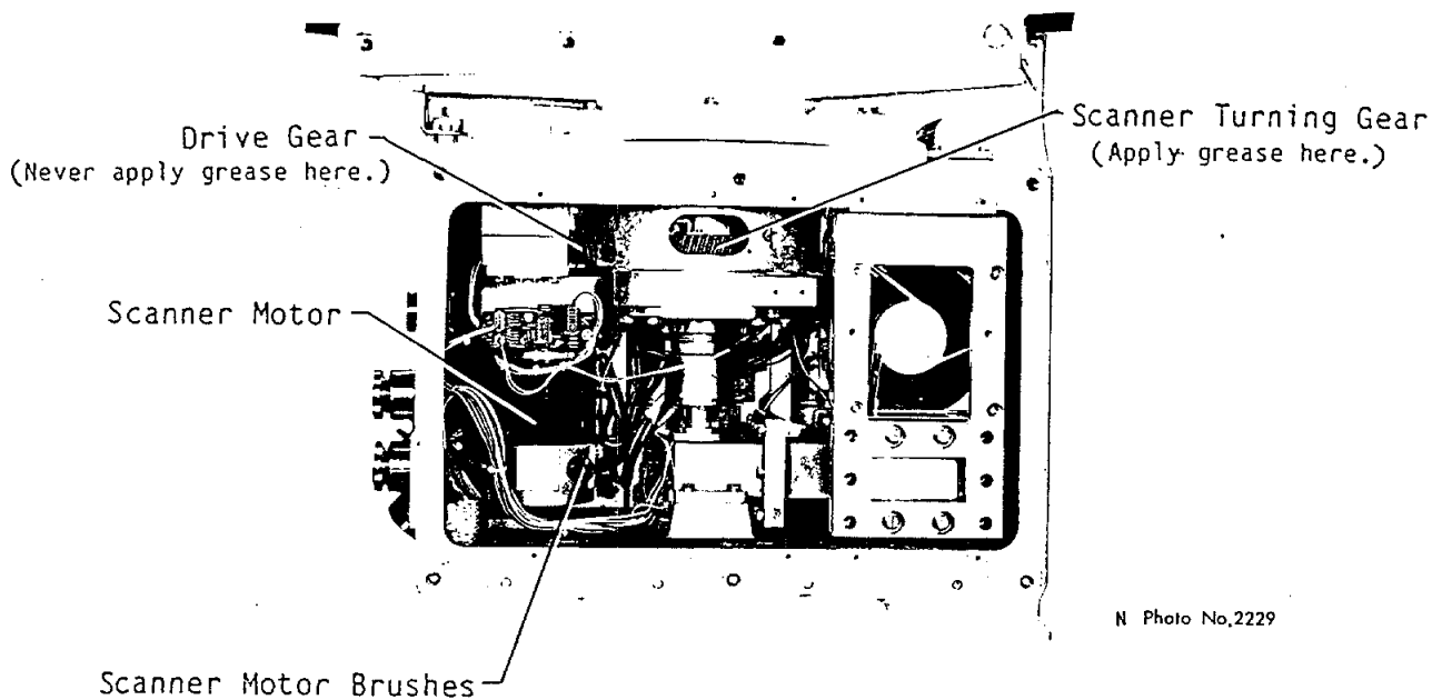
Figure 5-9 Scanner Unit, right side view (TX chassis removed)
