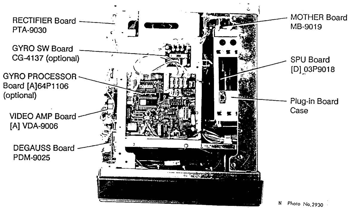
Figure 5-5 Display Unit, top view (cover opened)
