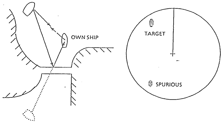
Figure 2-7 Indirect Echoes
