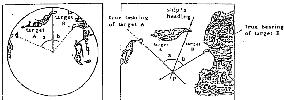
Figure 2-11 Position Fixing Using Two Bearings
