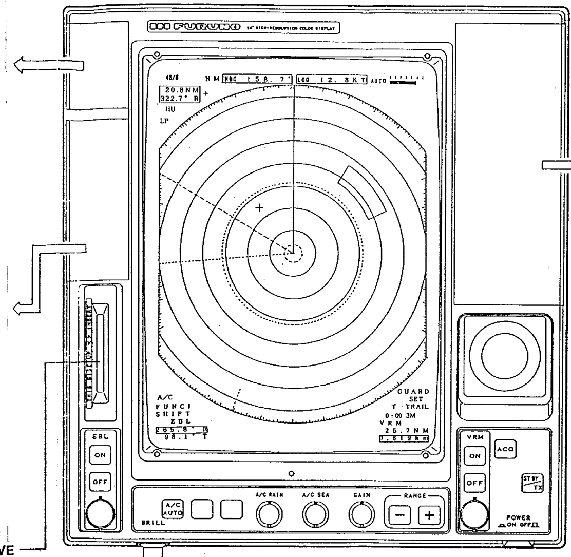
Figure 1-24 Display Unit
