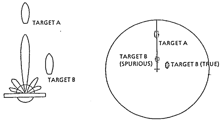
Figure 2-5 Side-lobe Echoes
