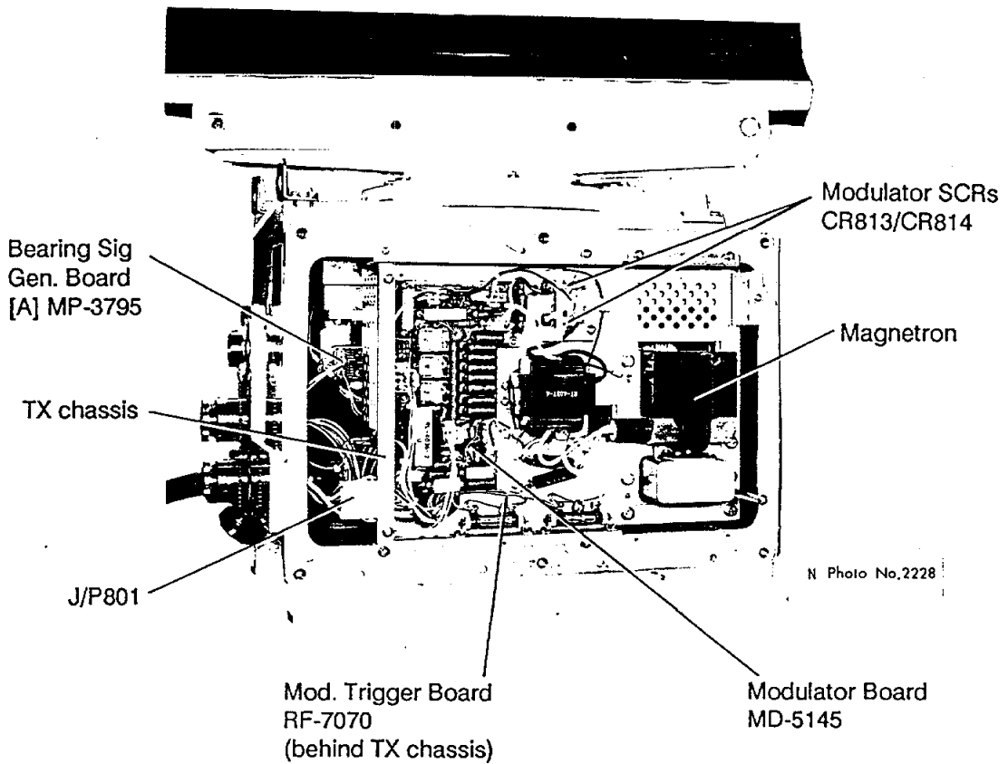
Figure 5-8 Scanner Unit, right side view (shield cover removed)
