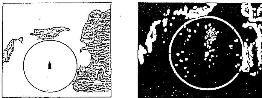
Figure 2-8 Navigation Chart and Corresponding Radar Picture
