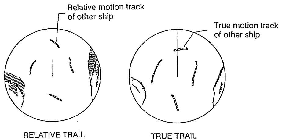
Figure 1-15 Echo Trailing
