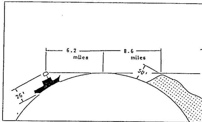
Figure 2-2 Radar Horizon
