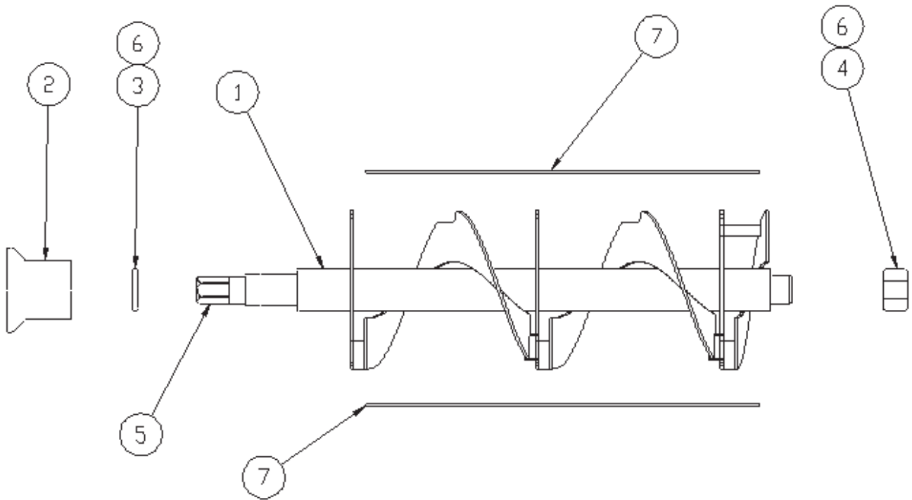
AUGER ASSEMBLY
